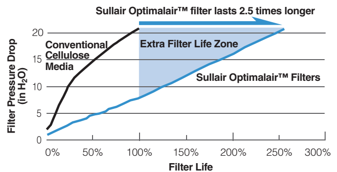
Filter Soot Life Test Results for Sullair
